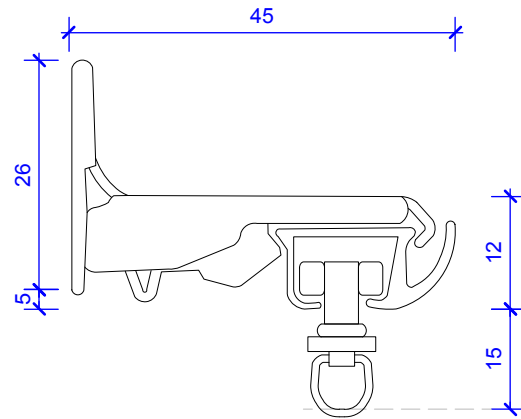
SERIES 58 SLIMLINE Fixed 35mm Projection Bracket No 5851
