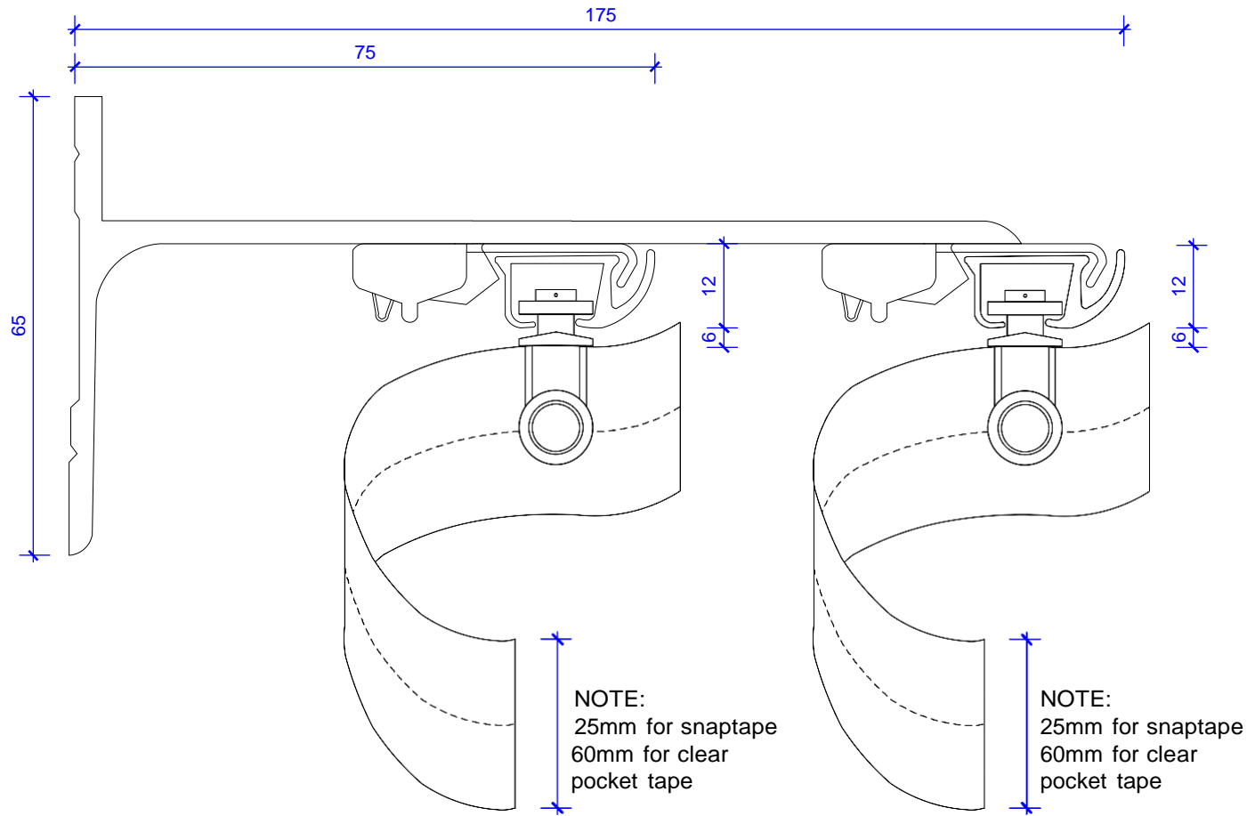
SERIES 58 SLIMLINE S-FOLD Double Support Bracket No 5855S
