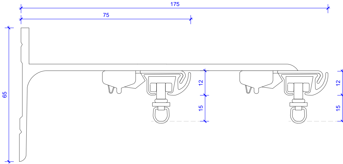
SERIES 58 SLIMLINE Double Support Bracket No 5855S
